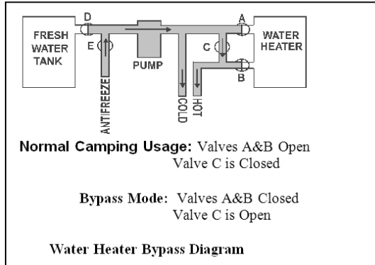
Factory installed water heater bypass
