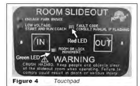
Figure 4 Touchpad
