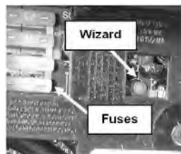
Wizard Button & Reverse Protection Fuses
